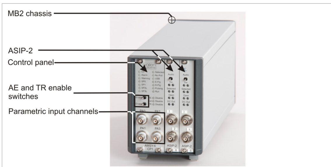
Figure 3: Front side of MB2 with front panel elements: ASIP-2 (chapter 3), AE-enable and TR-enable switch (2.5.1) and parametric input channels (2.5.2).
