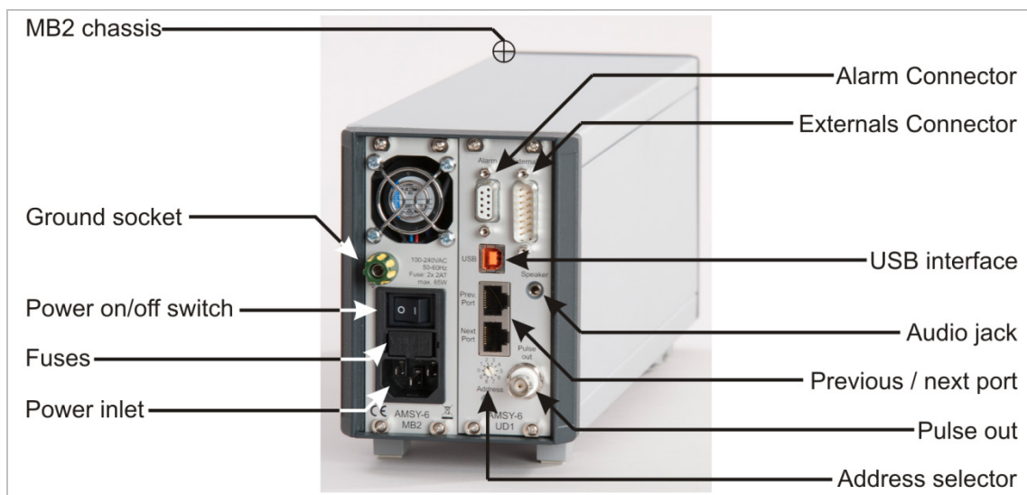
Figure 5: Rear side of MB2 with back panel elements: grounding post, power on/off switch (2.6.8), power inlet (2.2), alarm connector (2.6.2), externals connector (2.6.1), USB interface (2.6.6), audio jack (2.6.3), previous/next port (2.6.5), pulse out (2.6.7) and address selector (2.6.4).
