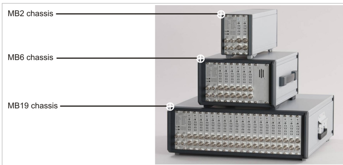
Figure 2: MB2, MB6 and MB19 chassis with 4, 12 and 38 AE-channels, respectively.
