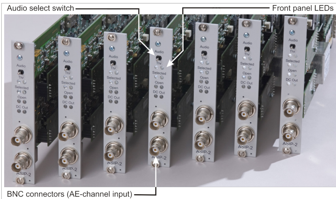
Figure 6: ASIP-2 with front panel elements: audio select switch, LEDs and BNC connectors
